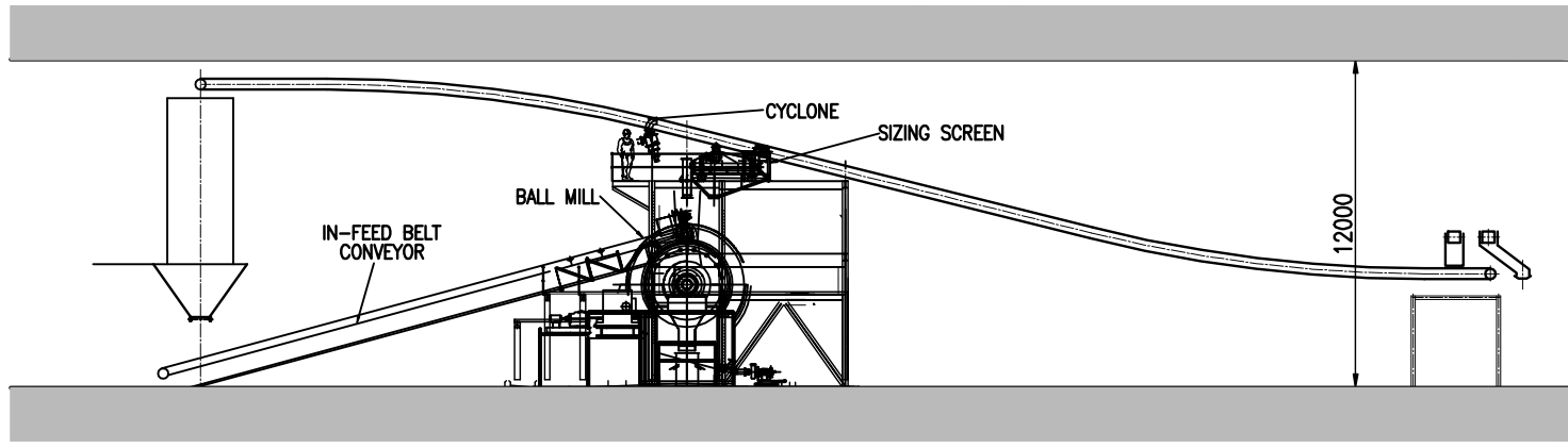
ELEVATION C-C : SCALE 1:200
