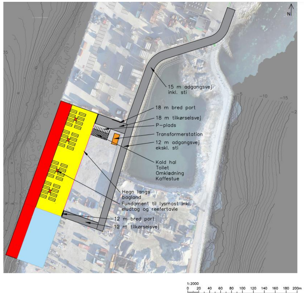
Figur 4-2 Qeqertaq Avallermi umiarsualiviup allineqarnissaata titartarneqarnera
