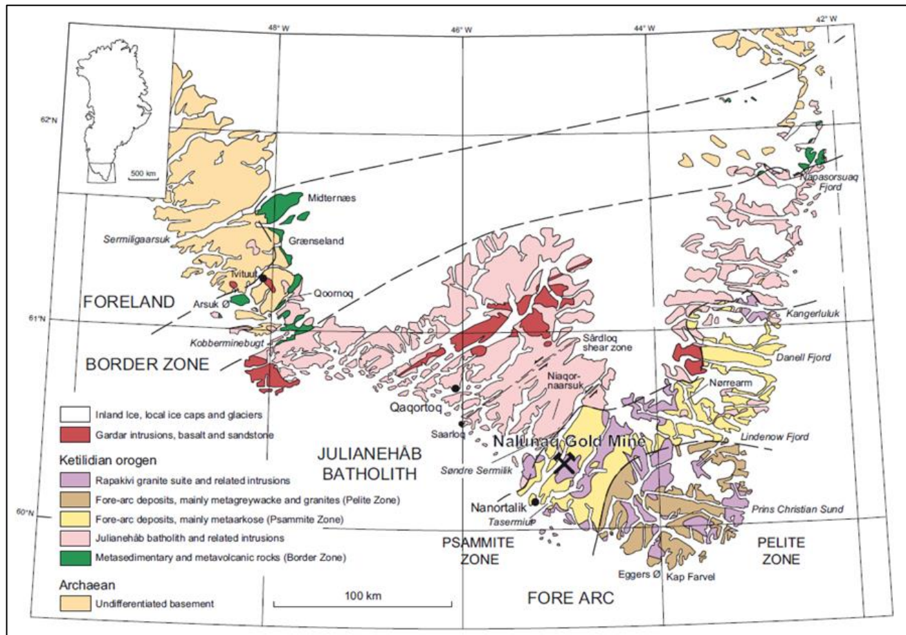
Takussutissiaq 3: Geological Map of Southern Greenland with the location of the Nalunaq Mine (from Secher et al., 2008)
