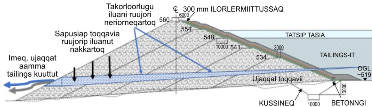
Ilusiliaq 50 Takorloorlugu ruujorit aseqqoqalernerat ([110] - Ilusiliaq 3.2)
