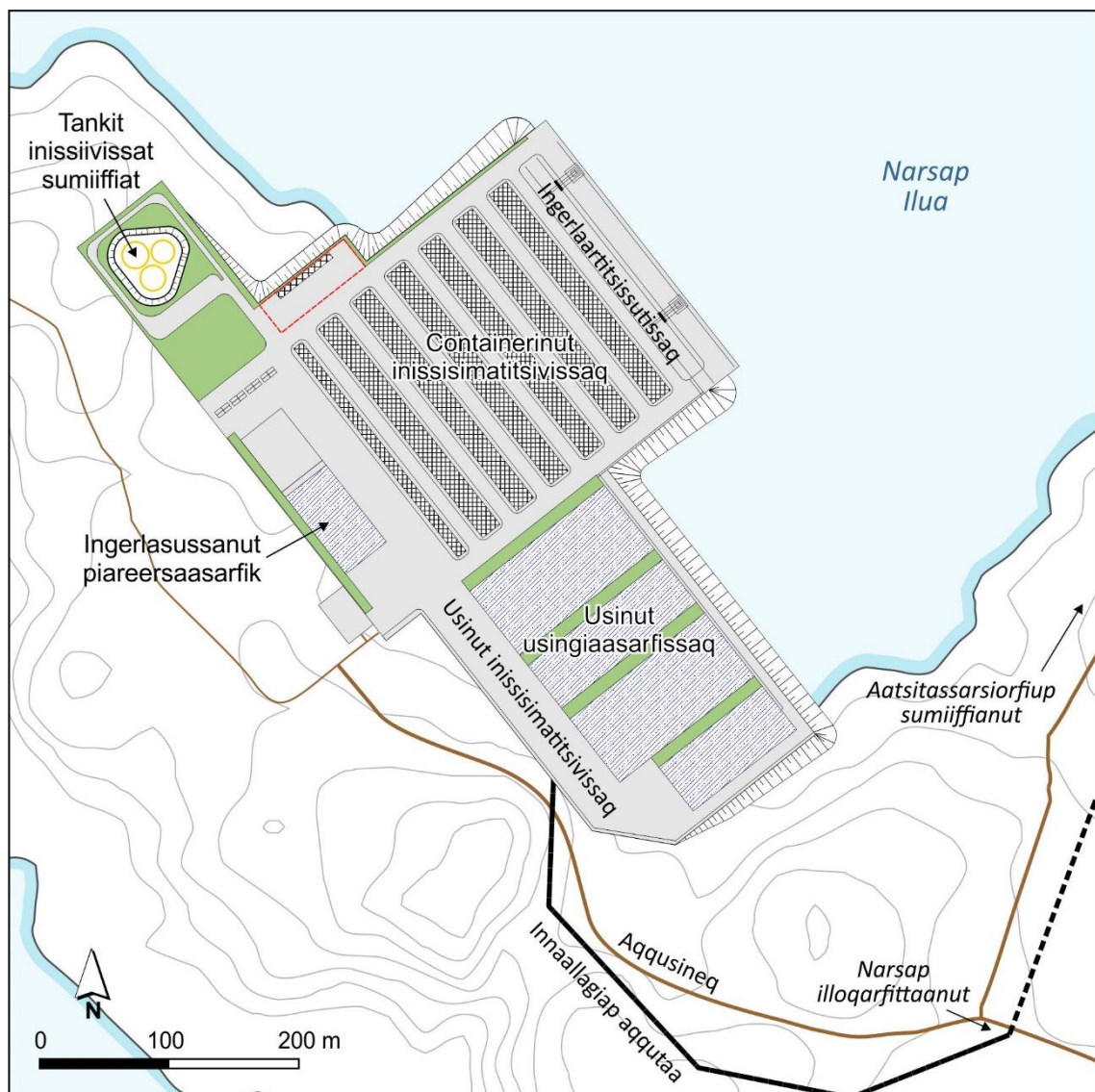
Ilusiliaq 22 Umiarsualiviup ilusiligaanera
