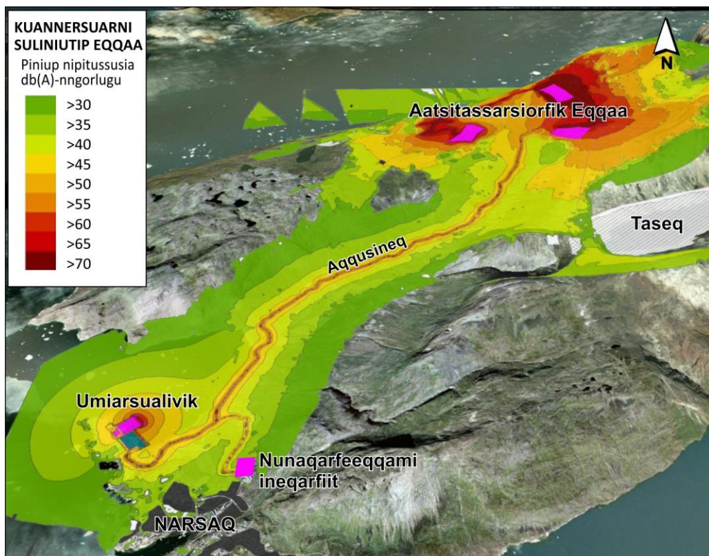
Takussutissiaq 7-8 Suliniummi nipiliornerup tamakkerlugu 3D-nngorlugu takusassiarineqarnera (Najoqqutaq: Orbicon, 2015)
