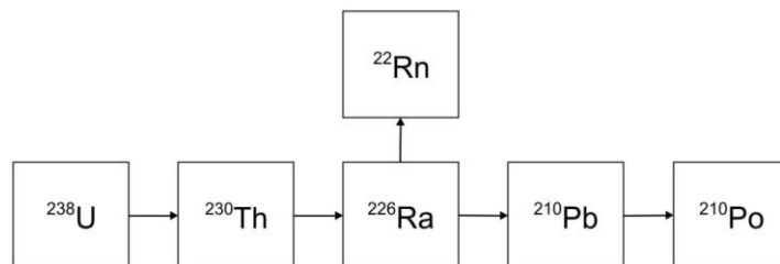
U-238-miit qinngornermit aseqqukut erseqqissumik takutinneri (Najoqqutaq: Arcadis, 2015)
