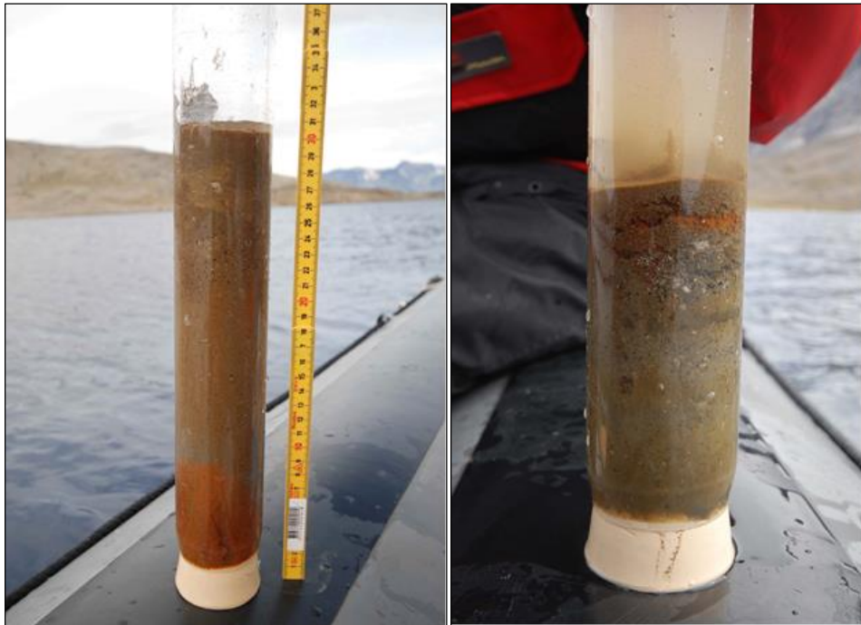
Ass. 6.9 Fostersø-miit kinnganernik misiligutit (talerpiani station 1 saamianilu station 2)
